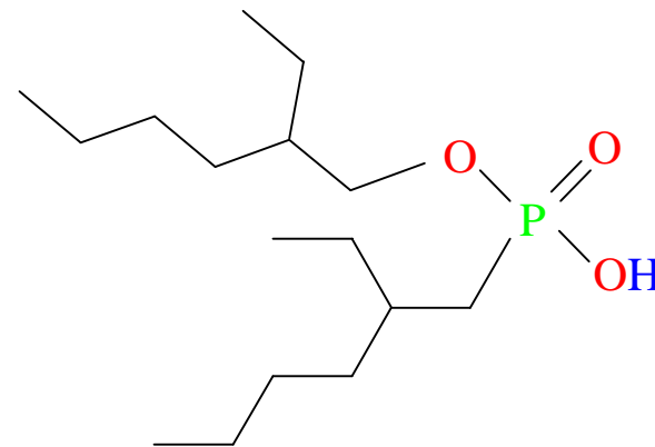
HEH[EHP] (LN2)
