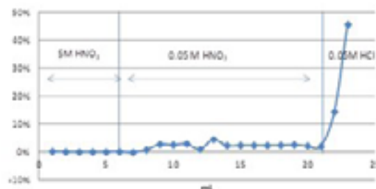
Ac elution study on 1mL TK221 Resin cartridge (100 – 200 \mu\text{m} ), 0.05M \text{HNO}_3 . Data courtesy of N. Vajda et al.
