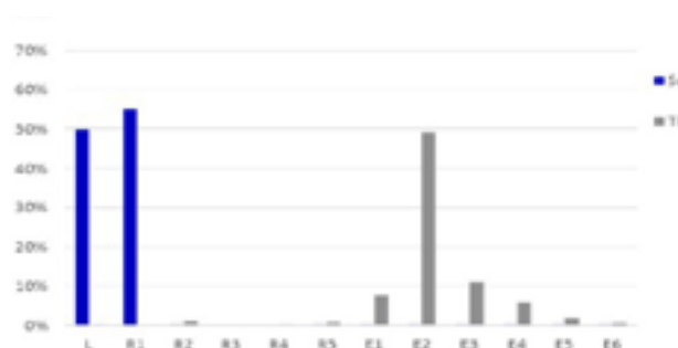
Ti/Sc separation on ZR Resin (0.3mL), fractions analysed by ICP-MS
