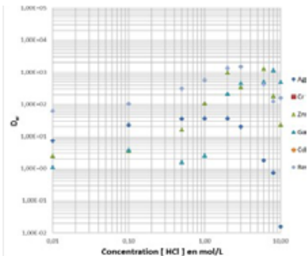
D_w values of selected elements on TK221 and TK222 in HCl
