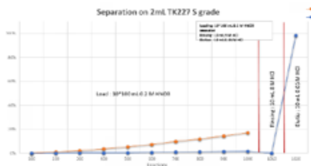
Elution study, 1L sea water, loading from 0.2M \text{HNO}_3 , Y separation, 2mL TK227 Resin cartridge
