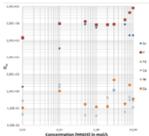
D_W values, TK227, selected elements, \text{HNO}_3
