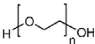
PolyEthyleneGlycol (PEG).
