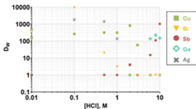
D_w values, TK250 Resin, selected elements, HCl
